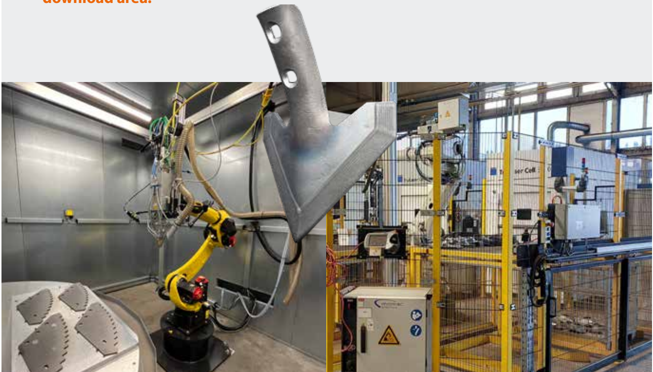
Laser cladding for knives (left), multifunction laser for coatings (right)
